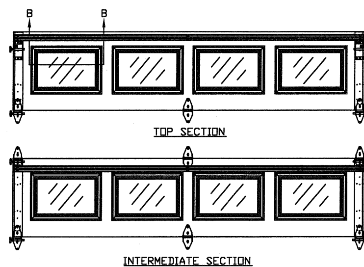
SHORT PANEL IMPACT GLAZING FASTENER DETAIL N.T.S.
